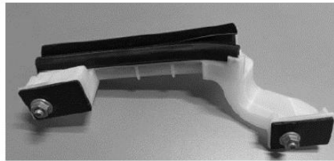
Front & Rear Door Window Guide Channel
