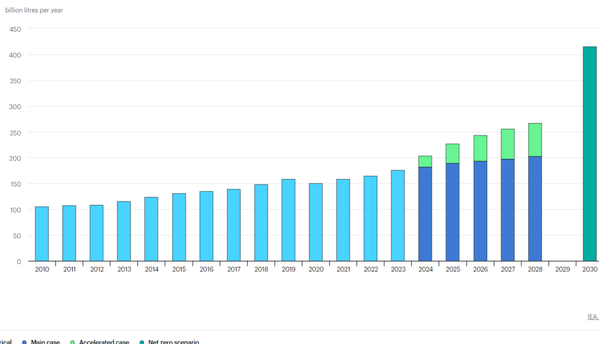
Global biofuel demand, main case, accelerated case and in the Net Zero Scenario, 2010-2030
