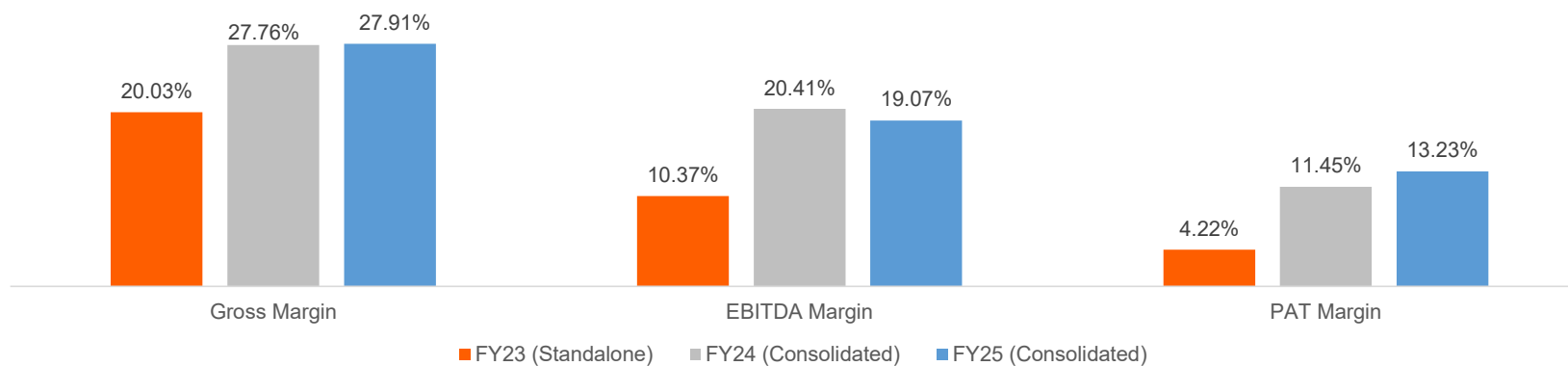
Operational Margins (%)
