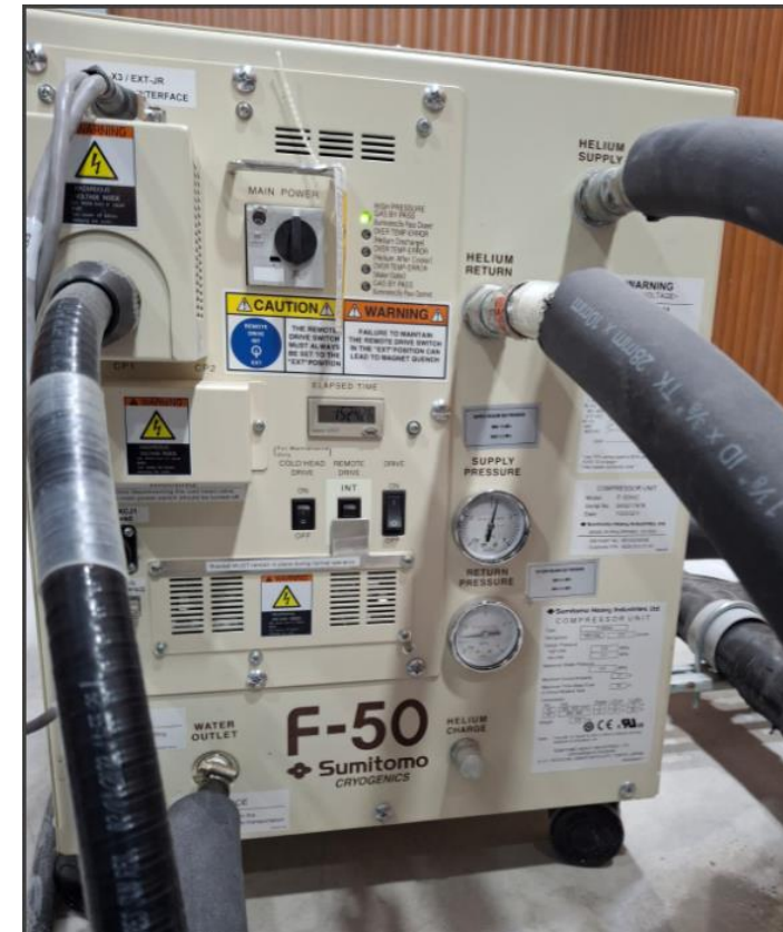
Helium Compressor
