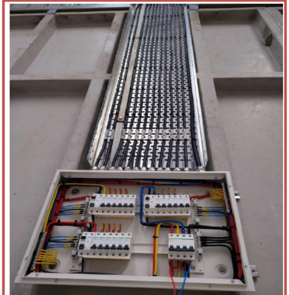
QC GOOD PRACTICE DB DARESSING, CABLE DARESSING
