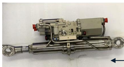
Actuator assemblies for LCA Tejas
