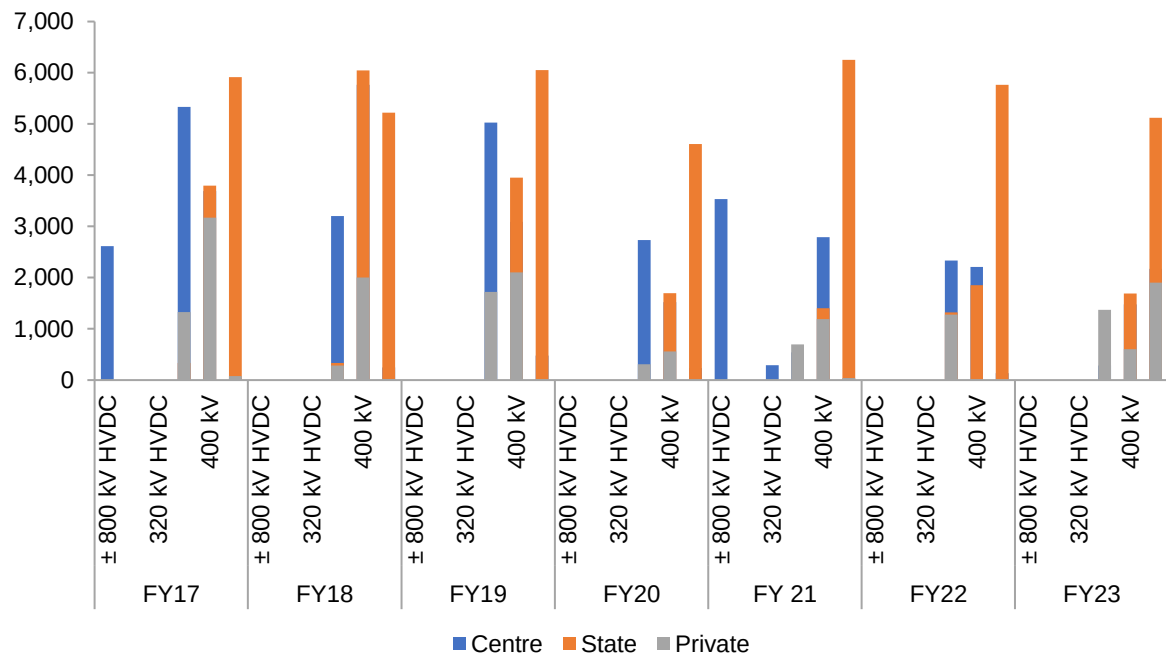
Transmission capacity addition at different voltage levels (fiscals 2017-2023)
