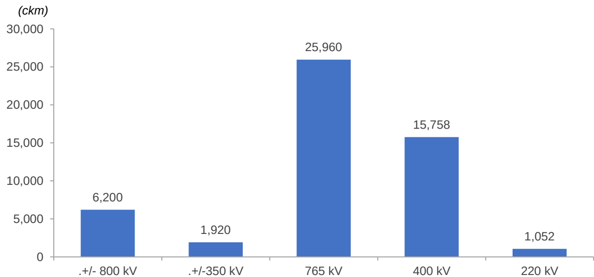
Outlook for voltage-wise line additions by 2030
