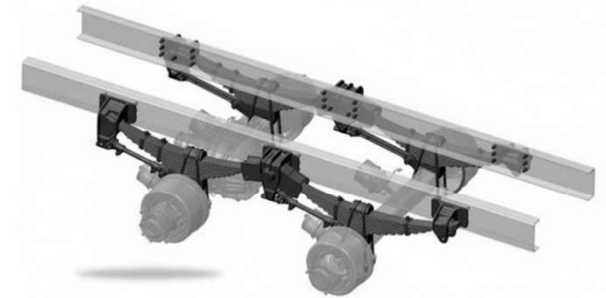
Slipper Suspension
