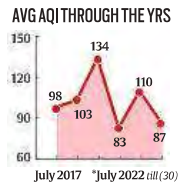
With the rainfall this month, the AQI has remained in the 'satisfactory' category for 24 out of 30 days of the month till Saturday. Ashish/Saha
