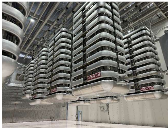
Valves hall at the converter station in Mumbai
