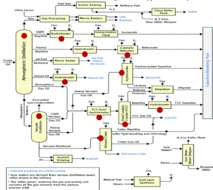
Exhibit 4.2: Process flow diagram of a typical refinery
