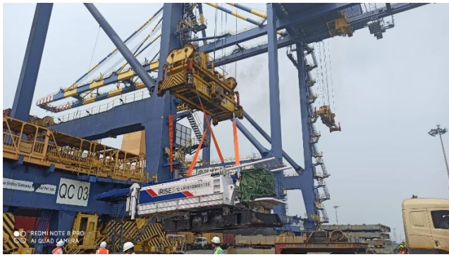
Breakbulk On Container Vessel Weight :- 48 Tons Each, Length :- 14 meter, Width :- 3.30 meter, Height :- 3.10 meters
